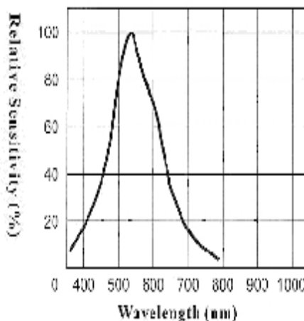
Spectral Response
